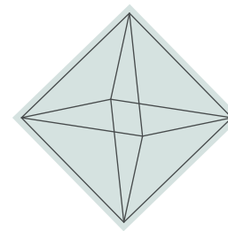
OCTAHEDRON
