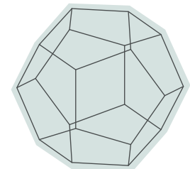
DODECAHEDRON
