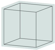
HEXAHEDRON
